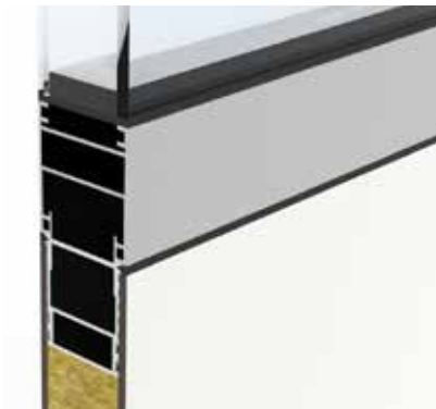
Window with 55 profile th.48 mm
